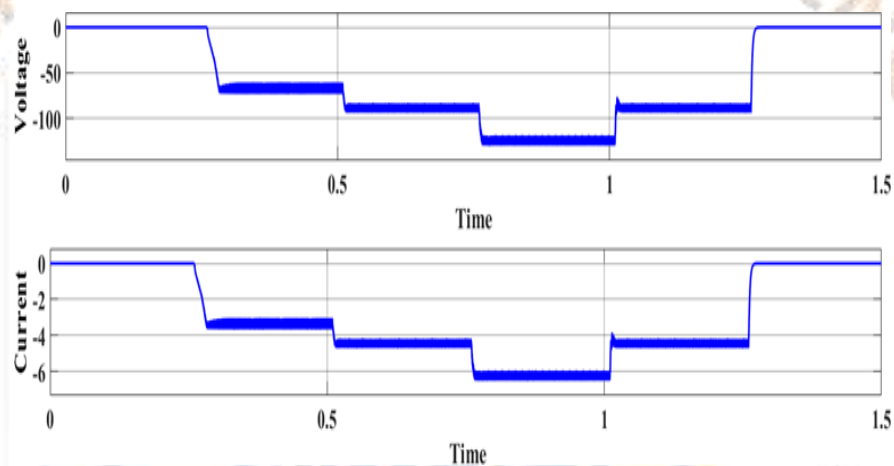
Figure 9. The output of the buck-boost converter
