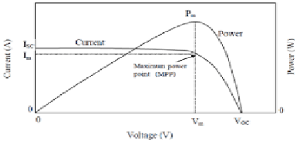
Figure 6. Characteristics of the solar cell for (b) pv
