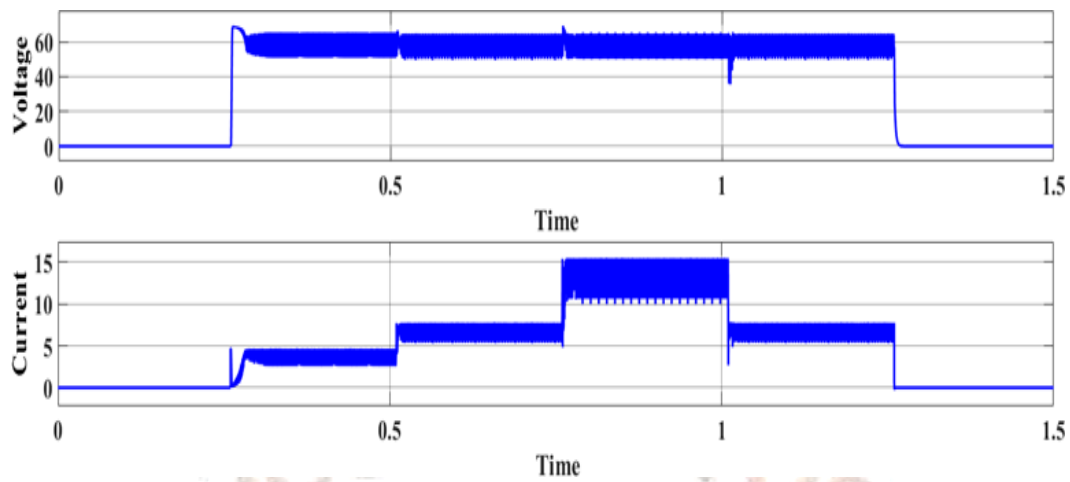
Figure 8. The output of the PV panel
