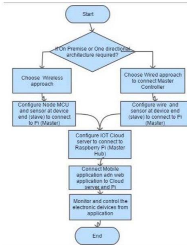
Fig. 8. Flowchart of the algorithm
