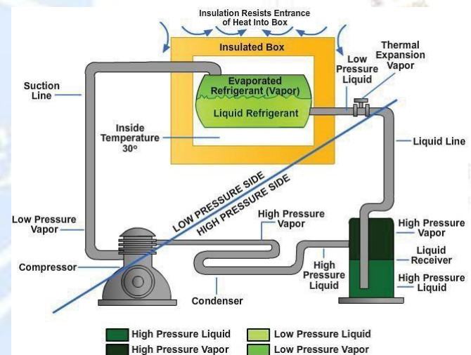
Figure 1.0 Refrigeration cycle
