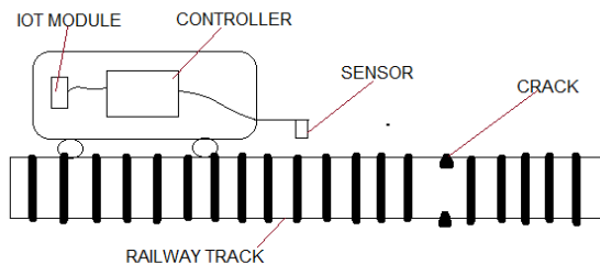
Figure 5. Structural Diagram
