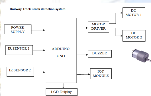
Figure 4. Block Diagram
