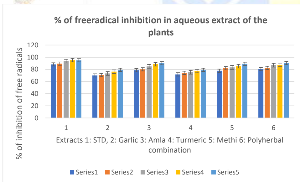
Fig. No 01: In vitro antioxidant activity of the plants and combined extracts (polyherbal extract) in aqueous extract
