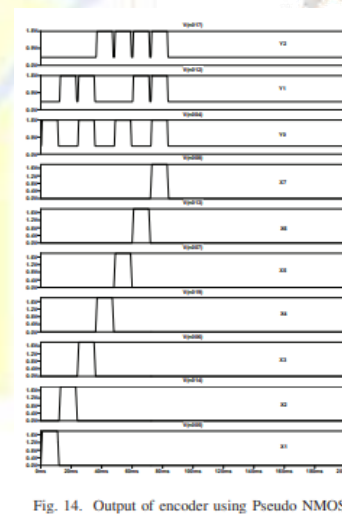
Fig. 14. Output of encoder using Pseudo NMOS
