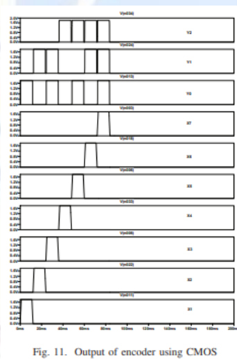
Fig. 11. Output of encoder using CMOS
