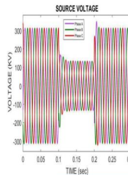
SOURCE VOLTAGE WITH FAULT OF EXISTING SYSTEM
