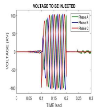
VOLTAGE TO BE INJECTED IN PROPOSED SYSTEM
