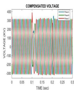
COMPENSATED VOLTAGE OF PROPOSED SYSTEM
